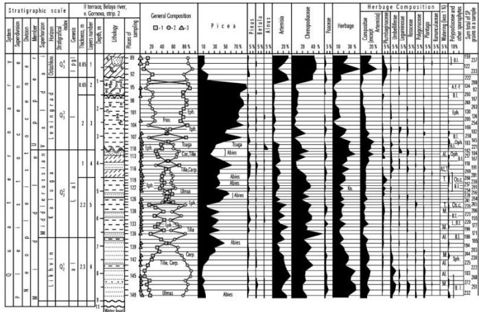
Fig. 5. Gornova locality. Deposits and percentage pollen curves of the main taxa from the interval Middle–Upper Pleistocene (after G. Danukalova and L. Alimbekova).
