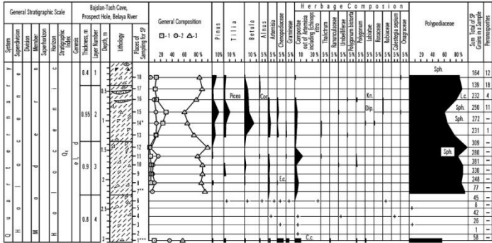
Fig. 3. Bajdan-Tash cave. Deposits and percentage pollen curves of the main taxa from the interval Upper Pleistocene–Holocene (after G. Danukolova, A. Yakovlev, and L. Alimbekova).
