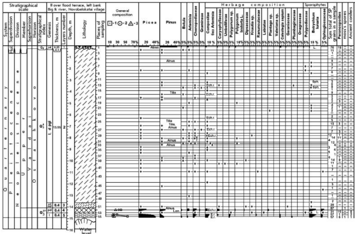
Fig. 4. Novobekokatay locality. Deposits and percentage pollen curves of the main taxa from the Upper Pleistocene (after G. Danukolova and L. Alimbekova).
